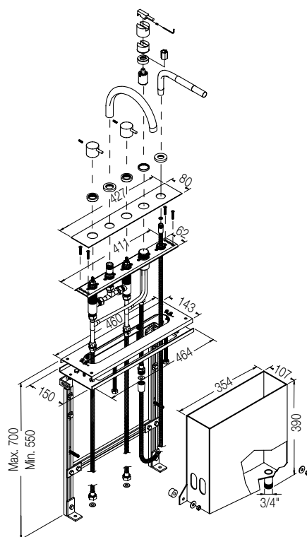
Komplet system (BK system)
